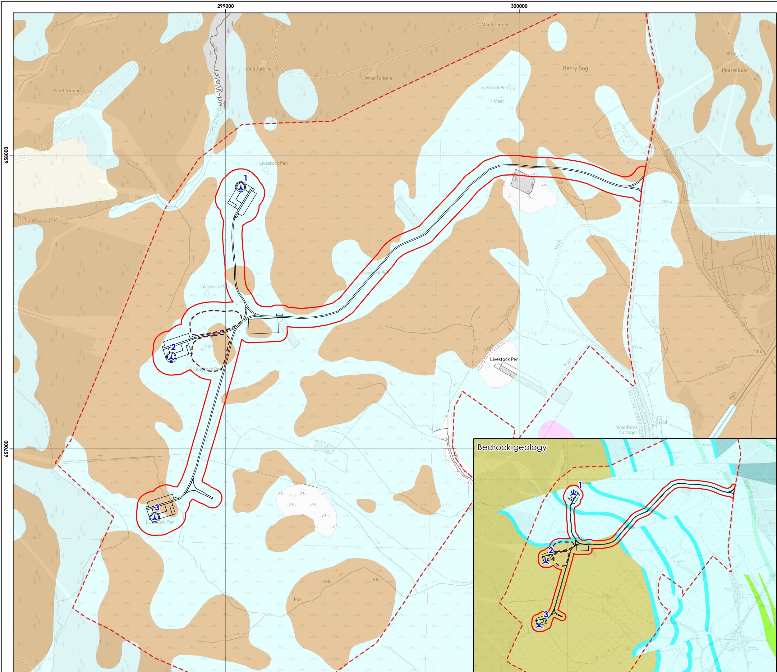
Figure 10-2 Superficial Geology
