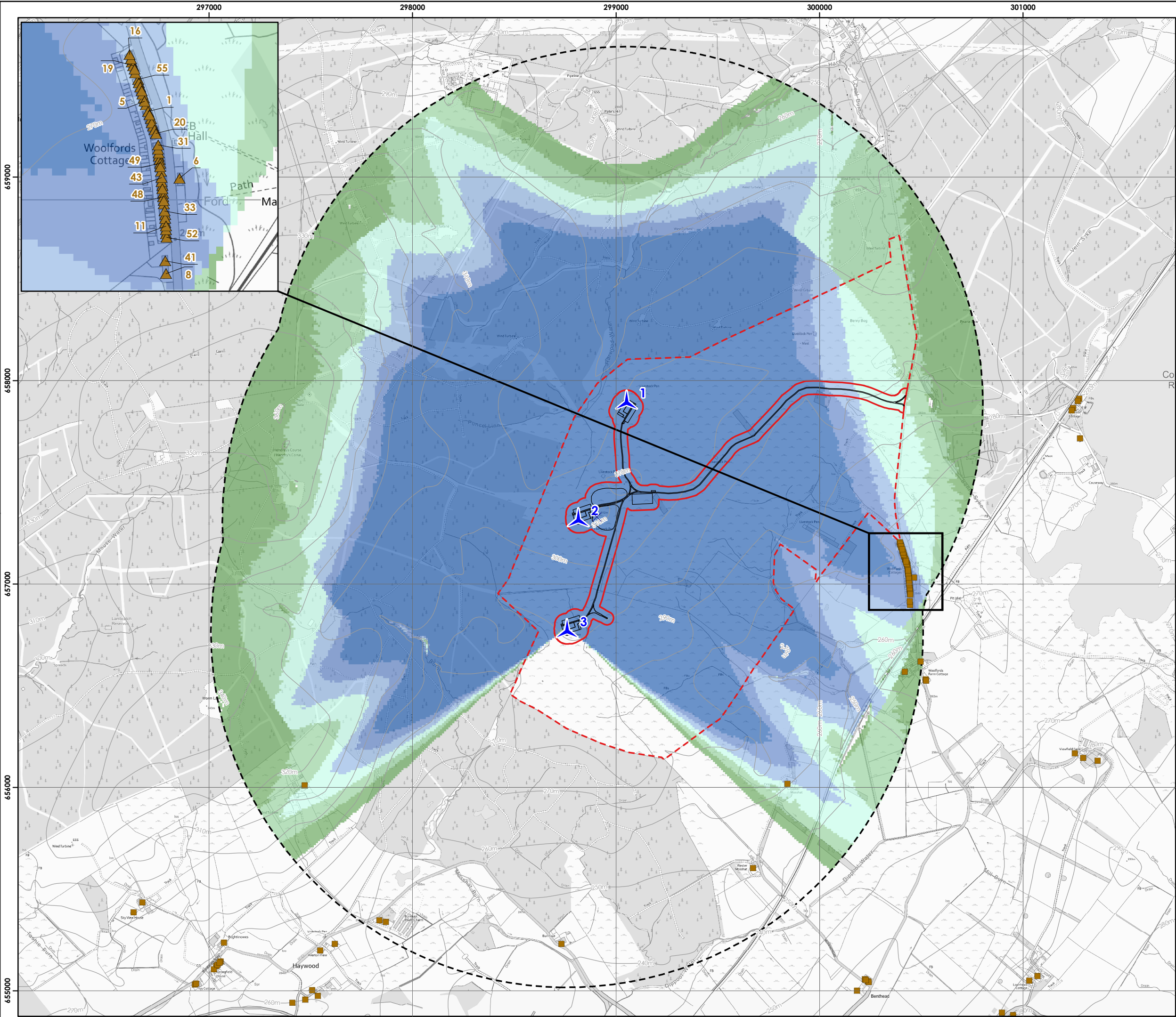
Figure 12-2 Shadow Flicker
