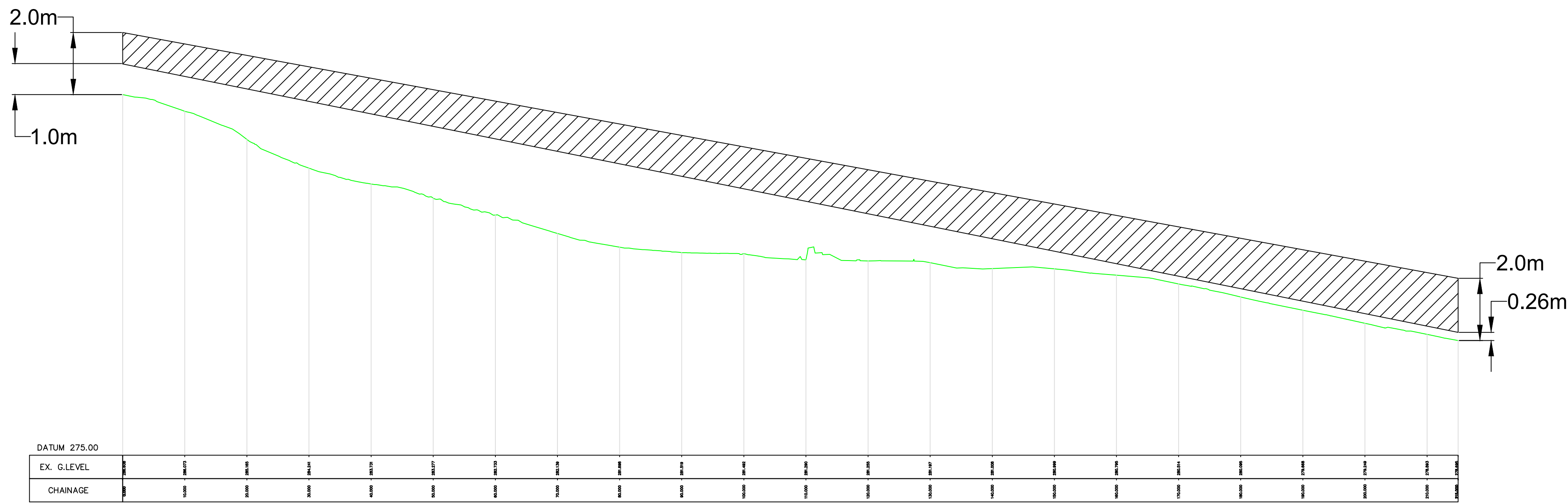
LONG SECTION (South Visibility 4.5m)
