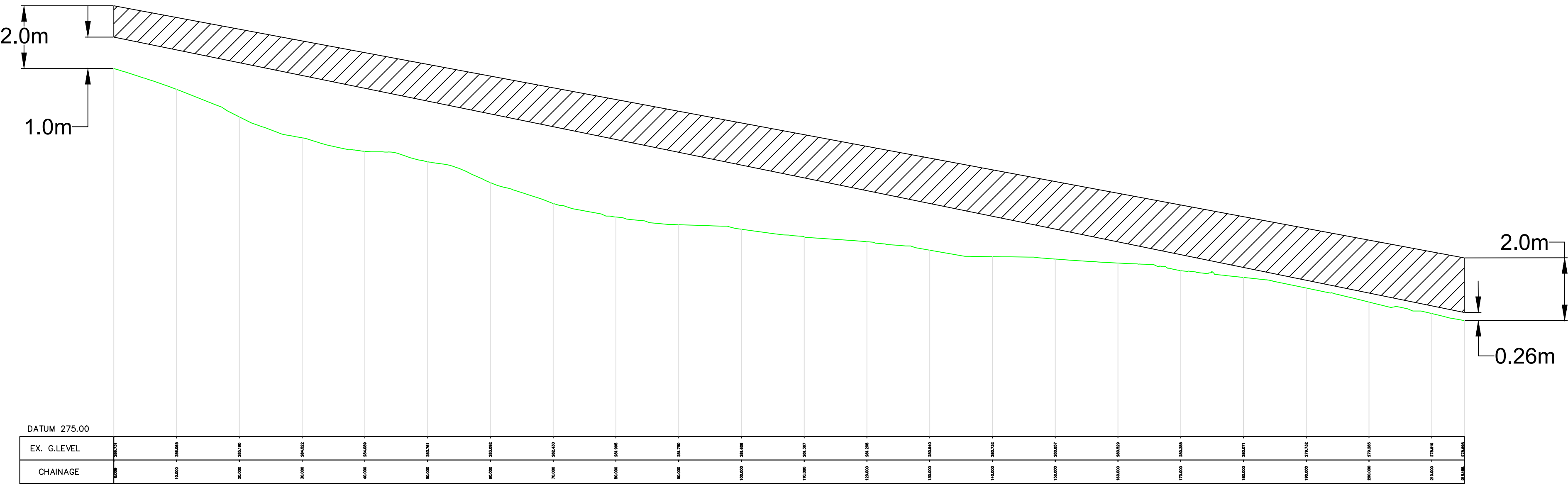
LONG SECTION (South Visibility 9.0m)
