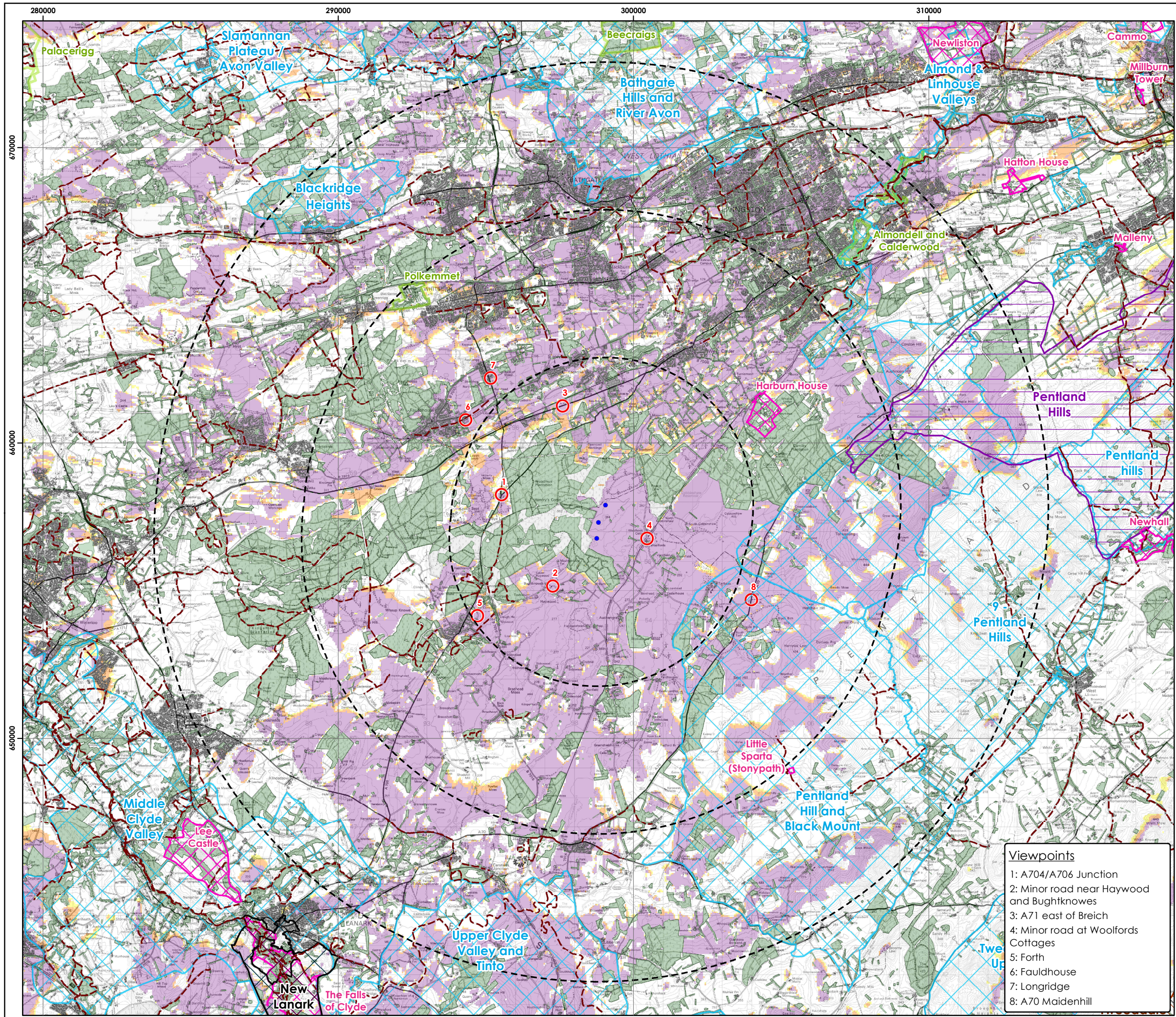
Figure 5-2 15km Screened Blade Tip ZTV with Landscape Designations
