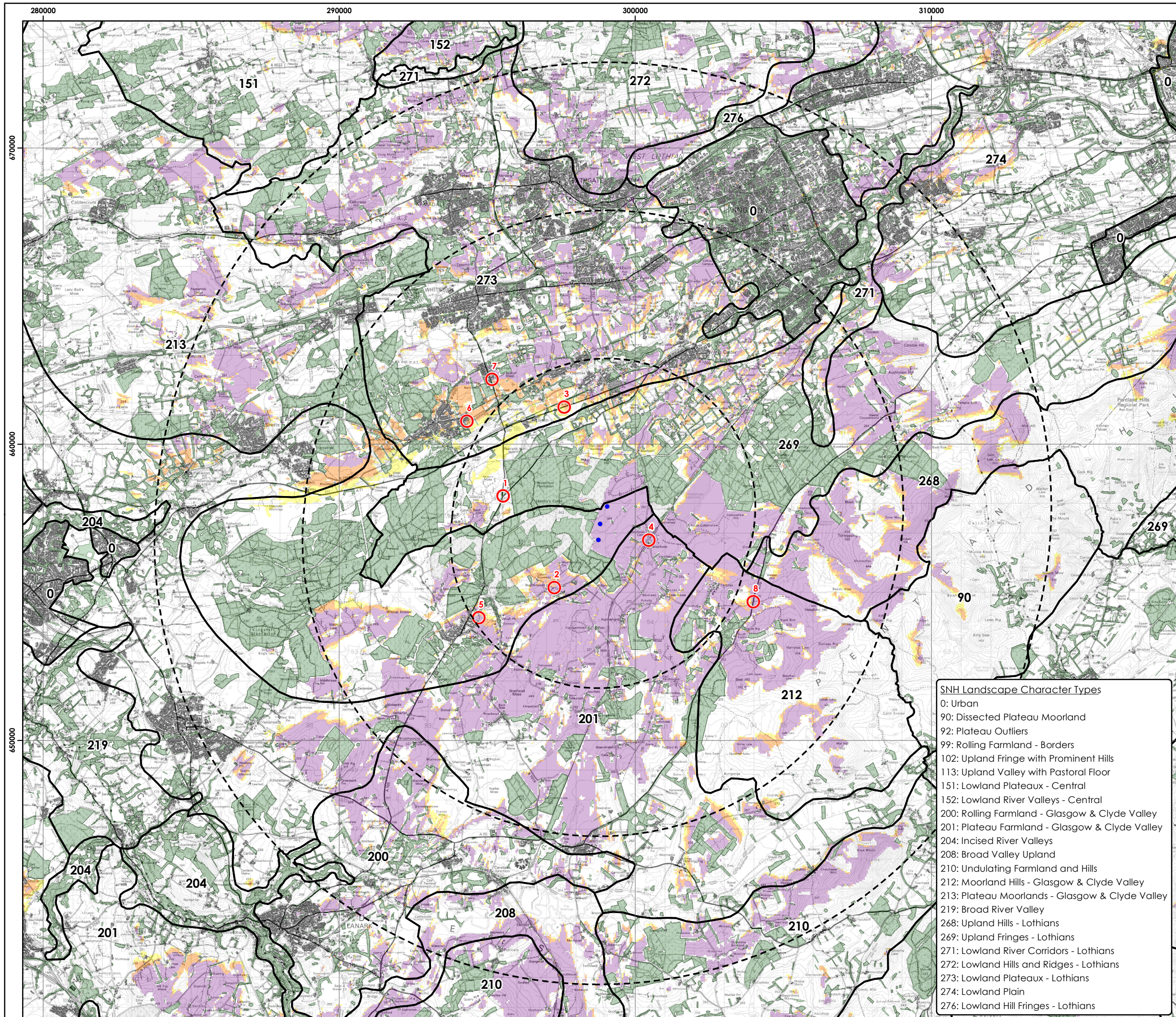
Figure 5-4 15km Screened Hub Height ZTV with Landscape Character Types
