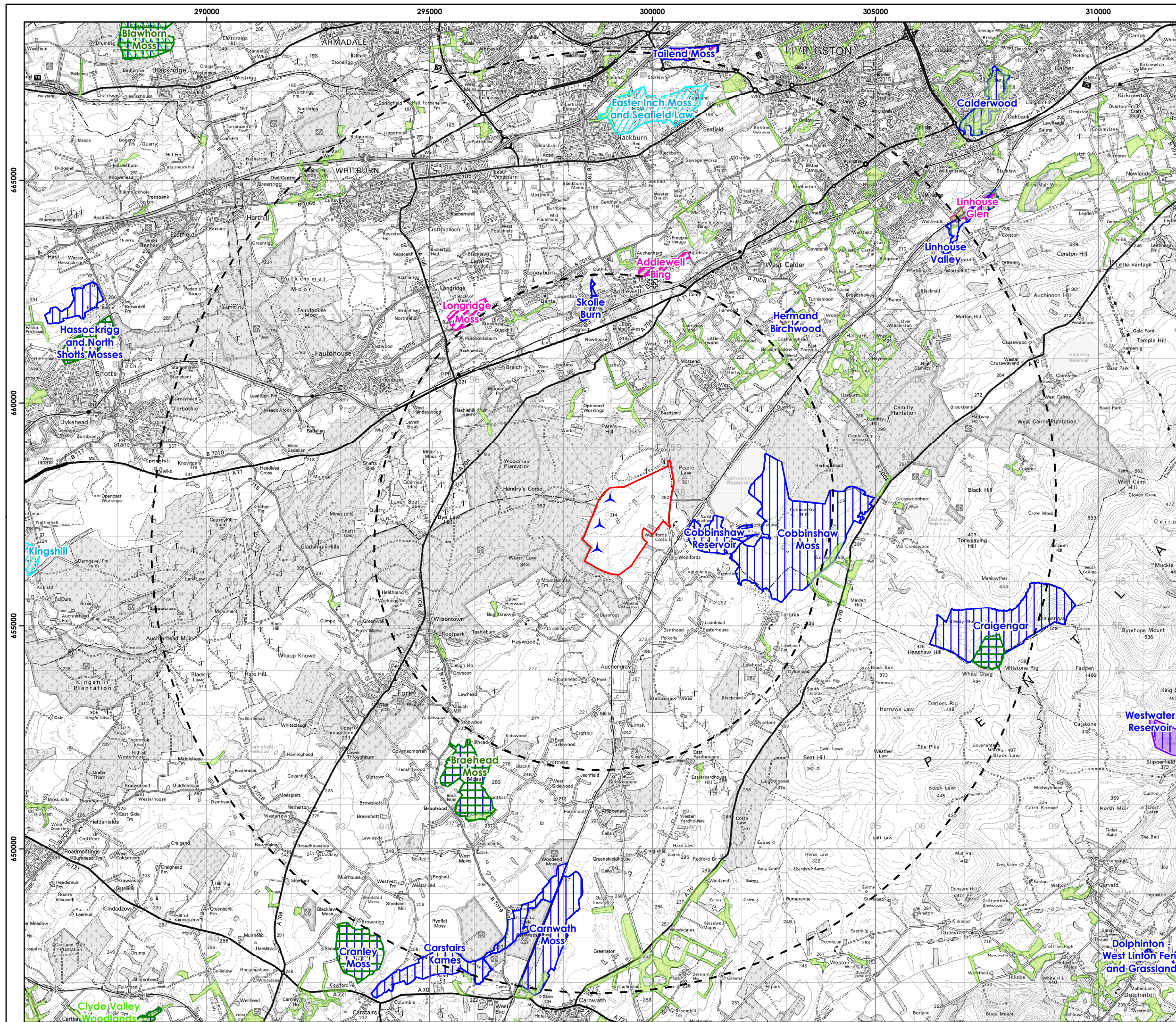
Figure 6-1 Designated Sites within 10km
