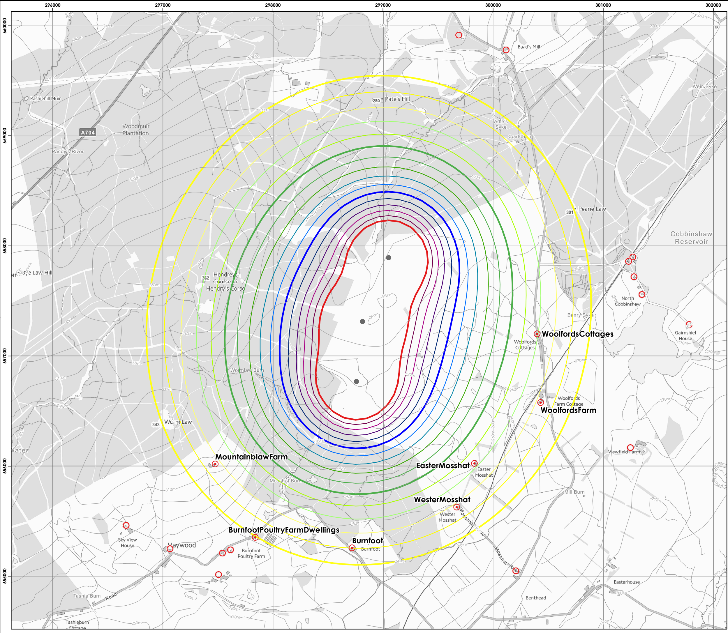
Figure 8-1 Predicted Operational Noise Levels for Proposed Varied Development at 8 m/s
