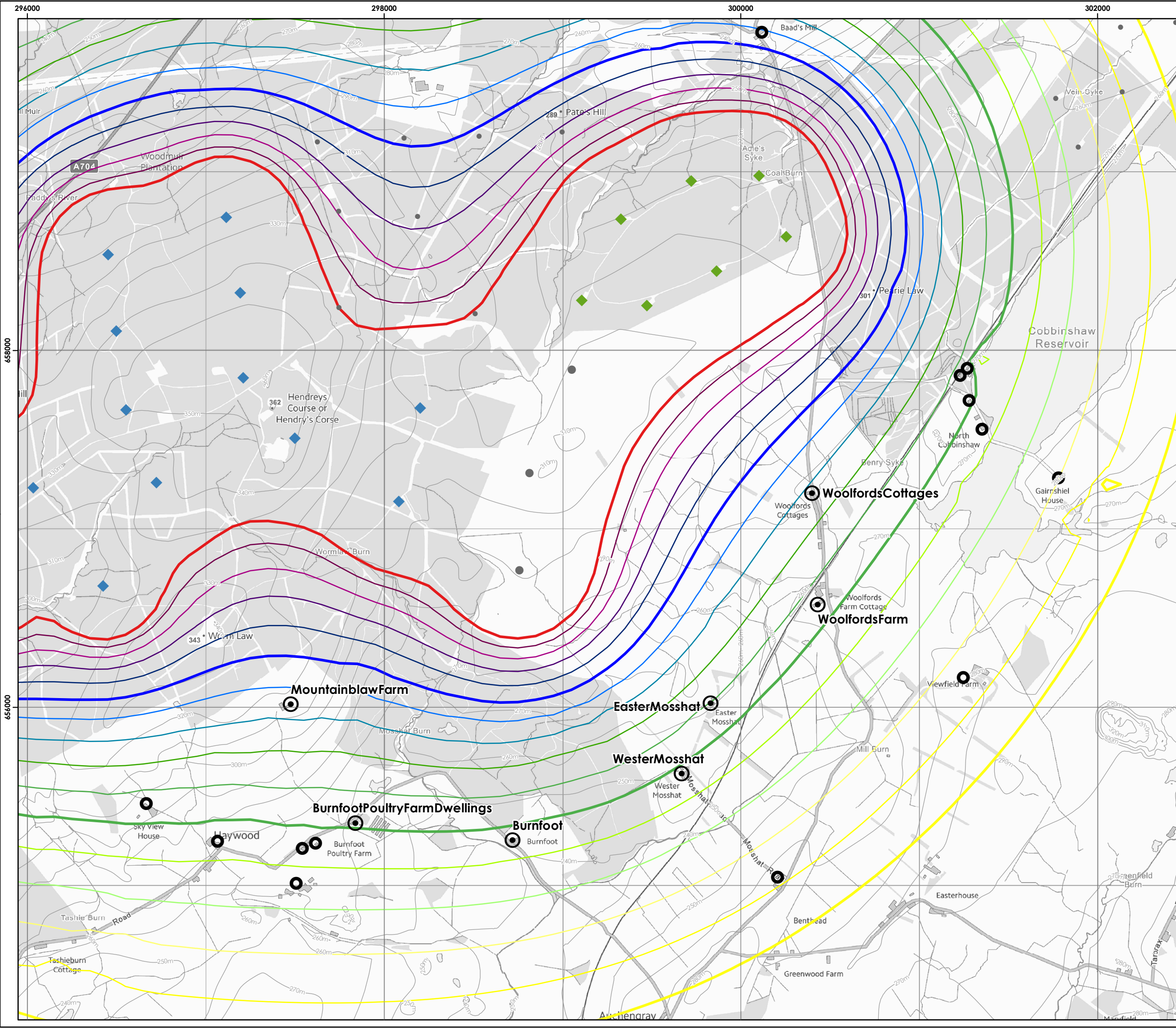
Figure 8-2 Predicted Cumulative Operational Noise Levels at 8 m/s
