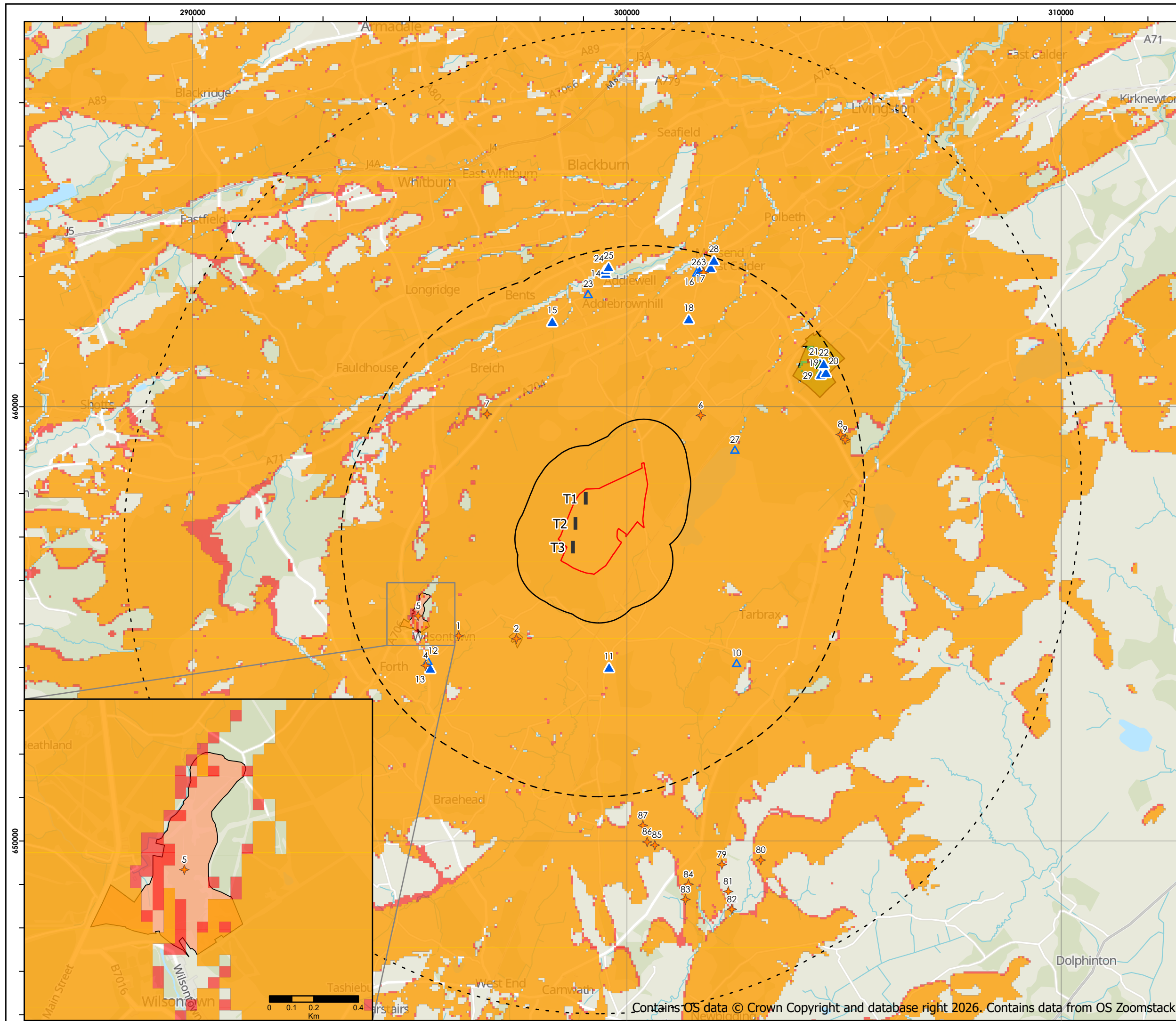
Figure 9-4 Comparative Zone of Theoretical Visibility
